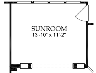
Opt. Sunroom
