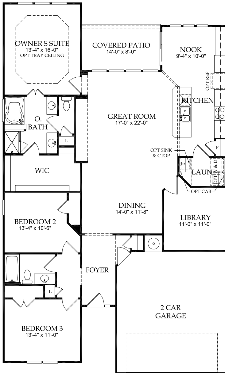
First Floor
